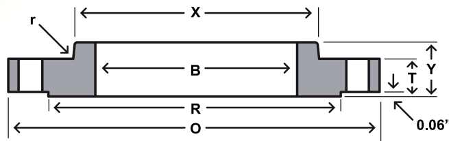
INDUSTRY STANDARD CLASS 150 SERIES "A" SLIP-ON FLANGES (BOLTING MATCHES)
