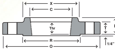
THREADED
