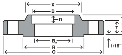
SOCKET WELD
