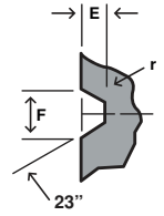
GROOVE DETAIL
