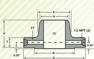
RAISED FACE
