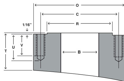
TANGENTIAL MOUNT
